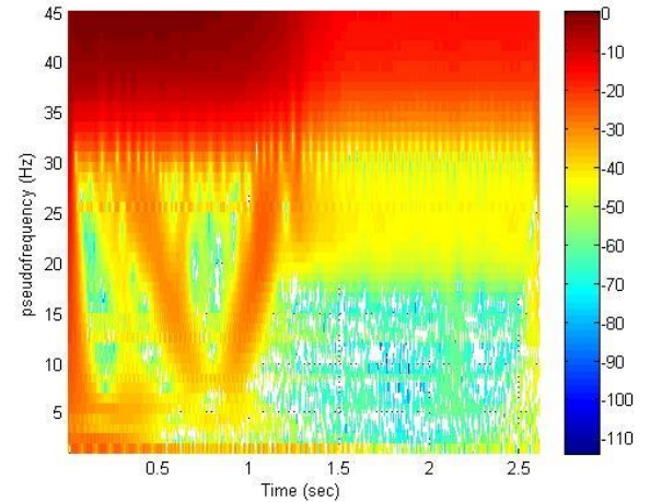
Fig. 3. Time-(pseudo)frequency plane for a motor with both mixed-eccentricity (35% static and 35% dynamic) and one broken bar created using the Morlet complex wavelet.
