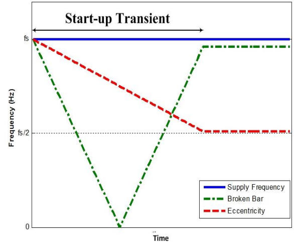
Fig. 1. Approximate evolution of the instantaneous frequency of faulty components during start-up.
